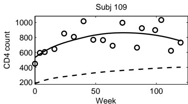
Figure 17.9 Type 1 SPME Modeling of the ACTG 388 Data: Raw Data (circles), Population Fits (dashed curves) and Individual Fits (solid curves) for Six Selected Subjects
