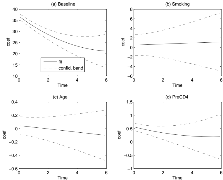
Figure 17.4 Type 3 SPME Modeling of the CD4 Data: Fitted Coefficient Functions (solid curves) with 95% Pointwise Standard Deviation Bands (dashed curves)
