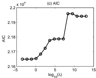
Figure 17.7 Type 1 SPME Modeling of the ACTG 388 Data: Smoothing Parameter Selection
