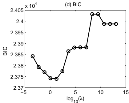
Figure 17.7 Type 1 SPME Modeling of the ACTG 388 Data: Smoothing Parameter Selection
